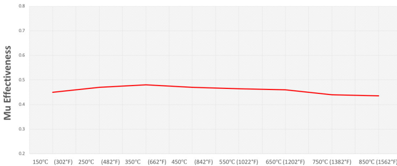
Circo M119 Friction vs Temperature
